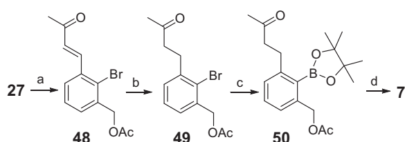
Scheme 6. Synthesis of compound 7 . Reagents and conditions: (a) \text{Ph}_3\text{P}=\text{CHCOCH}_3 , \text{PhMe} , 90^\circ\text{C} , 1 h; (b) \text{H}_2 , 10% \text{Pd/C} , EA, rt, 1 h; (c) \text{Pin}_2\text{B}_2 , \text{Pd}(\text{dppf})\text{Cl}_2 , KOAc, 1,4-dioxane, 103^\circ\text{C} , 16 h; (d) \text{NaOH} , MeOH, rt, 1 h, then HCl, THF.
