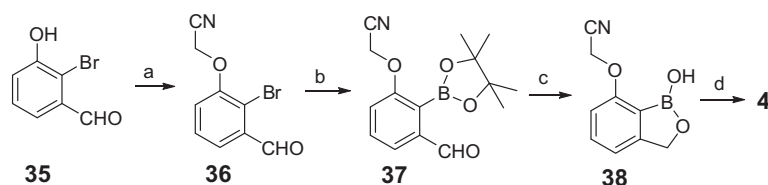
Scheme 4. Synthesis of compound 4 . Reagents and conditions: (a) BrCH 2 CN, K 2 CO 3 , DMF, rt 20 h; (b) Pin 2 B 2 , Pd(dppf)Cl 2 , KOAc, 1,2-DME, 90 °C 16 h; (c) NaBH 4 , EtOH, rt, 1 h, then HCl; (d) HCl (g), MeOH, H 2 O, rt, 1 h.
