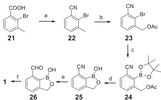
Scheme 1. Synthesis of compound 1 . Reagents and conditions: (a) (1) i -PrOC(O)Cl, TEA, DCM, 0 °C, 10 min, (2) NH_4OH , 0 °C, 2 min, (3) (CNCl)_3 , rt, 16 h; (b) (1) NBS, Bz_2O_2 , CCl_4 , reflux, 16 h, N_2 , (2) KOAc, DMF, 80 °C, 1 h; (c) Pin_2B_2 , Pd(dppf)Cl 2 , KOAc, 1,4-dioxane, reflux, 16 h, N_2 ; (d) (1) NaOH, MeOH, rt, 2 h, (2) HCl, H 2 O, THF, rt, 50 min; (e) Raney Ni, HCOOH, H 2 O, 100 °C, 1 h; (f) 2,2-dimethyl-1,3-dioxane-4,6-dione, HCOOH, TEA, reflux, 15 h.
