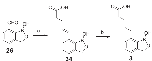
Scheme 3. Synthesis of compound 3 . Reagents and conditions: (a) Ph 3 PCH 2 CH 2 CH 2 COOH bromide, NaH, DMSO, rt, 4 h; (b) H 2 , Pd/C, EtOAc, rt, 1 h.
