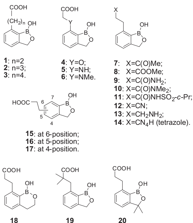
Figure 1. Chemical structures of the benzoxaborole compounds synthesized 6 during a structure–activity relationship investigation for the discovery of a new class of antimalarial agents by variations of the side-chain length (1–3), one of the side-chain CH_2 with hetero atoms such as O or N (4–6), the side chain functional group (7–14), the position of attachment of the side chain on the benzoxaborole scaffold (15–17), the oxaborole ring size (18) and additional substitution changes on the \alpha -carbon next to the carboxylic group (19) and to oxaborole 3-position carbon (20).
