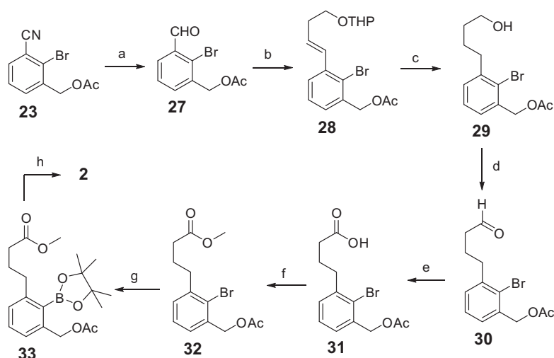
Scheme 2. Synthesis of compound 2 . Reagents and conditions: (a) Raney Ni, HCO 2 H, H 2 O, 100 °C, 1 h; (b) Ph 3 P=CHCH 2 CH 2 OTHP, THF, –78 °C to rt, 20 h; (c) (1) H 2 , Pd/C, EtOAc, rt, 1 h, (2) 2 N HCl, EA, MeOH, H 2 O, 40 °C, 0.5 h; (d) (COCl) 2 , DMSO, DCM, –78 °C, 15 min, then TEA, rt, 2 h; (e) 2-methylbut-2-ene, NaClO 2 , NaH 2 PO 4 , t -BuOH, rt, 1.5 h; (f) MeI, K 2 CO 3 , DMF, rt, 1 h; (g) Pin 2 B 2 , KOAc, Pd(dppf)Cl 2 , KOAc, 1,4-dioxane, N 2 , 85 °C, 16 h; (h) (1) NaOH, MeOH, rt, 2 h, (2) HCl, H 2 O, THF, rt, 1 h.
