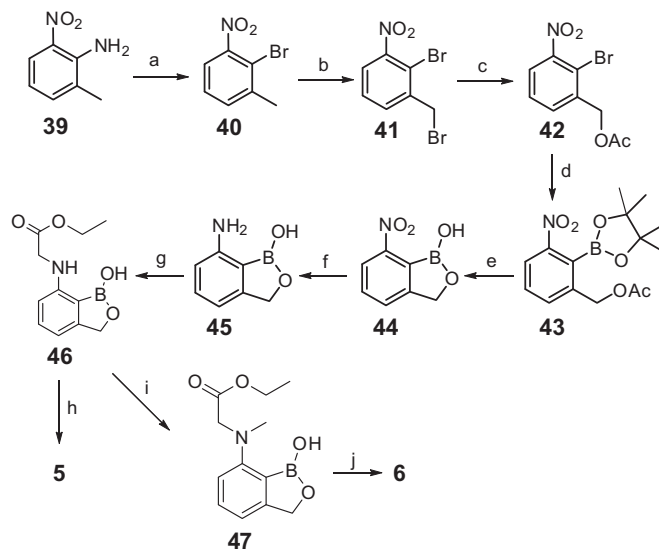
Scheme 5. Synthesis of compounds 5 and 6 . Reagents and conditions: (a) (1) NaNO 2 , 40% aq HBr, 0 °C, 1 h, (2) CuBr, 100 °C, 1 h; (b) NBS, CCl 4 , AIBN, reflux, 16 h; (c) NaOAc, DMF, 70 °C 16 h; (d) Pin 2 B 2 , Pd(dppf)Cl 2 , KOAc, 1,4-dioxane, 95 °C, 20 h; (e) NaOH, MeOH, rt, 24 h, then 5 N HCl, THF, 40 °C, 16 h; (f) H 2 , Pd/C, rt, 2.5 h; (g) ethyl 2-bromoacetate, K 2 CO 3 , DMA, rt, 16 h; (h) LiOH, THF/MeOH/H 2 O, rt, 2 h; (i) DMF, CH 3 I, K 2 CO 3 , DMF, rt, 2 h; (j) LiOH, THF/MeOH/H 2 O, rt, 2 h.
