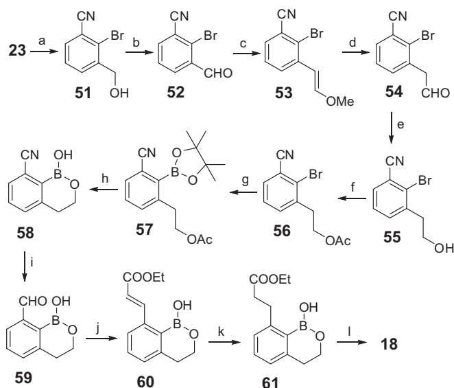
Scheme 8. Synthesis of compound 18 . Reagents and conditions: (a) \text{LiOH} , THF/MeOH/ \text{H}_2\text{O} , rt 1 h; (b) PCC, DCM, rt, 2 h; (c) \text{Ph}_3\text{PCH}_2\text{OME} chloride, t\text{-BuOK} , DMSO, 0^\circ\text{C} to rt, 16 h; (d) 6 N HCl, THF, reflux 1 h; (e) \text{NaBH}_4 , MeOH, rt, 1 h; (f) \text{CH}_3\text{COCl} , \text{Et}_3\text{N} , DCM, 0^\circ\text{C} , 2 h; (g) \text{Pin}_2\text{B}_2 , \text{Pd}(\text{dppf})\text{Cl}_2 , KOAc, 1,4-dioxane, \text{N}_2 , reflux, 2 h; (h) \text{NaOH} , MeOH, \text{H}_2\text{O} , then HCl, THF; (i) Raney Ni, \text{HCO}_2\text{H} , \text{H}_2\text{O} , 100^\circ\text{C} , 1 h; (j) \text{Ph}_3\text{PCH}_2\text{COOCH}_2\text{CH}_3 bromide, NaH, THF, 0^\circ\text{C} to rt, 16 h; (k) \text{H}_2 , Pd/C, EtOAc, rt, 2 h; (l) \text{NaOH} , MeOH, \text{H}_2\text{O} , rt, 16 h, then HCl.
