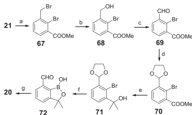
Scheme 10. Synthesis of compound 20 . Reagents and conditions: (a) (1) \text{SOCl}_2 , MeOH, reflux, 3 h, (2) NBS, \text{Bz}_2\text{O}_2 , \text{CCl}_4 , 80\text{--}85^\circ\text{C} , 5 h; (b) \text{CaCO}_3 , \text{H}_2\text{O} , 1,4-dioxane, 100^\circ\text{C} , 5 h; (c) silica gel, PCC, DCM, 0\text{--}5^\circ\text{C} , 3 h; (d) \text{HOCH}_2\text{CH}_2\text{OH} , p\text{-TsOH} , toluene, reflux, 5 h; (e) \text{MeMgBr} , THF, -10^\circ\text{C} to rt, 16 h; (f) n\text{-BuLi} , THF, -78^\circ\text{C} , 0.5 h, then \text{B}(\text{OMe})_3 , -78^\circ\text{C} to rt, 16 h, and finally HCl, \text{H}_2\text{O} , rt, 1 h; (g) 2,2-dimethyl-1,3-dioxane-4,6-dione, HCOOH, \text{Et}_3\text{N} , 100^\circ\text{C} , 12 h.
