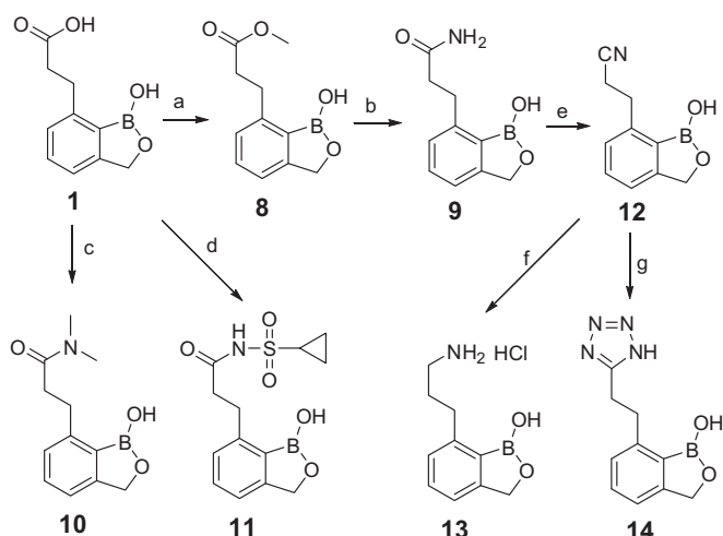
Scheme 7. Synthesis of compounds 8–14 . Reagents and conditions: (a) \text{MeI} , \text{K}_2\text{CO}_3 , DMF, rt, 1 h; (b) \text{NH}_4\text{OH} , MeOH, 50^\circ\text{C} , 16 h; (c) \text{Me}_2\text{NH HCl} , EDC HCl, DIPEA, HOAt, THF, DCM, rt, 3 h; (d) (1) CDI, THF, reflux, 1 h, (2) cyclopropanesulfonamide, DBU, rt, 16 h; (e) (\text{CNCl})_3 , DMF, rt, 16 h; (f) \text{H}_2 , Ni, \text{NH}_4\text{OH} , MeOH, rt, 1 h; (g) \text{NaN}_3 , \text{NH}_4\text{Cl} , DMF, 95^\circ\text{C} , 3 days.
