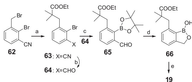
Scheme 9. Synthesis of compound 19 . Reagents and conditions: (a) \text{LiN}(i\text{-Pr})_2 , ethyl isobutyrate, -20^\circ\text{C} , 45 min; (b) Raney Ni, \text{HCO}_2\text{H} , \text{H}_2\text{O} , 100^\circ\text{C} , 1 h; (c) \text{Pin}_2\text{B}_2 , \text{Pd}(\text{dppf})\text{Cl}_2 , KOAc, 1,4-dioxane, \text{N}_2 , 103^\circ\text{C} , 16 h; (d) \text{NaBH}_4 , EtOH, 0^\circ\text{C} to rt, 1 h, then HCl; (e) \text{LiOH} , THF/MeOH/ \text{H}_2\text{O} , rt, 16 h, then HCl.
