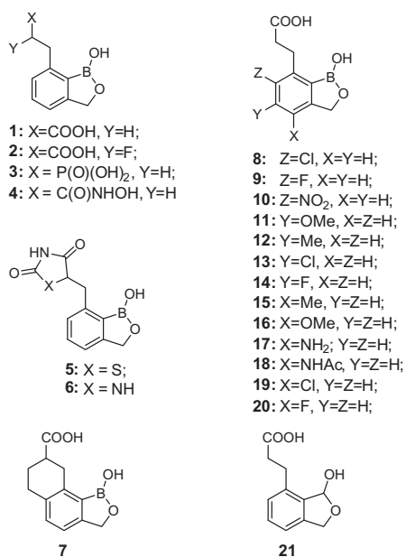
Figure 1. Chemical structures of the benzoxaborole compounds synthesized during a SAR investigation for the discovery of a new class of antimalarial agents by the side-chain variation (2–7), substituent change on the benzene ring (8–20) and removal of boron from five-membered oxaborole ring (21).
