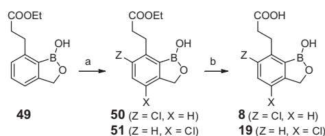
Scheme 4. Syntheses of compounds 8 and 19 . Reagents and conditions: (a) \text{SO}_2\text{Cl}_2 , AcOH, 50 °C, 16 h; (b) NaOH, THF, \text{H}_2\text{O} , rt, 2 h, then 1 N HCl.
