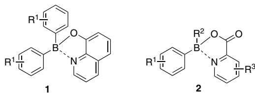
Figure 1. Diphenylborinic acid ester complexes.
