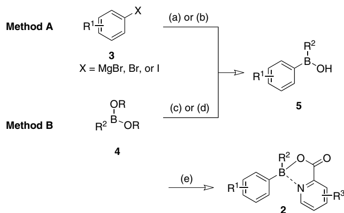
Scheme 1. Synthesis of borinic acid picolinate esters ( 2 ). Reagents and conditions: (a) \text{B}(\text{OMe})_3 (0.5 equiv), THF, 0^\circ\text{C} to rt (when X = \text{MgBr} ); (b) \text{BuLi} , \text{B}(\text{OMe})_3 (0.5 equiv), THF, -78^\circ\text{C} to rt (when X = \text{Br} ); (c) 3 ( X = \text{MgBr} ), THF, 0^\circ\text{C} to rt; (d) 3 ( X = \text{Br} ), \text{BuLi} , THF, -78^\circ\text{C} to rt; (e) R^3 -picolinic acid, EtOH, water, reflux.
